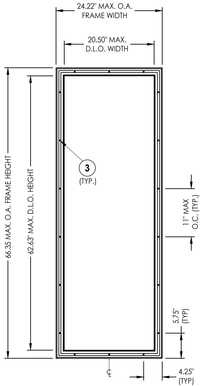
ODL LITE FRAME DETAIL "Traditional" Profile
