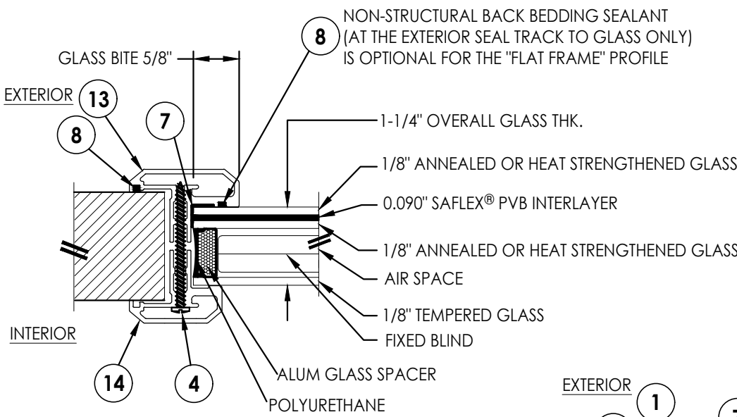
G5 GLAZING DETAIL ALUM SPACER w/ FIXED BLIND
